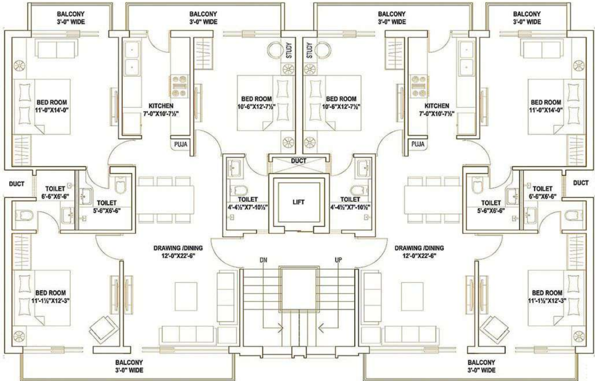
TYPICAL FLOOR PLAN SIZE = 30'-0" x 60'-0"
