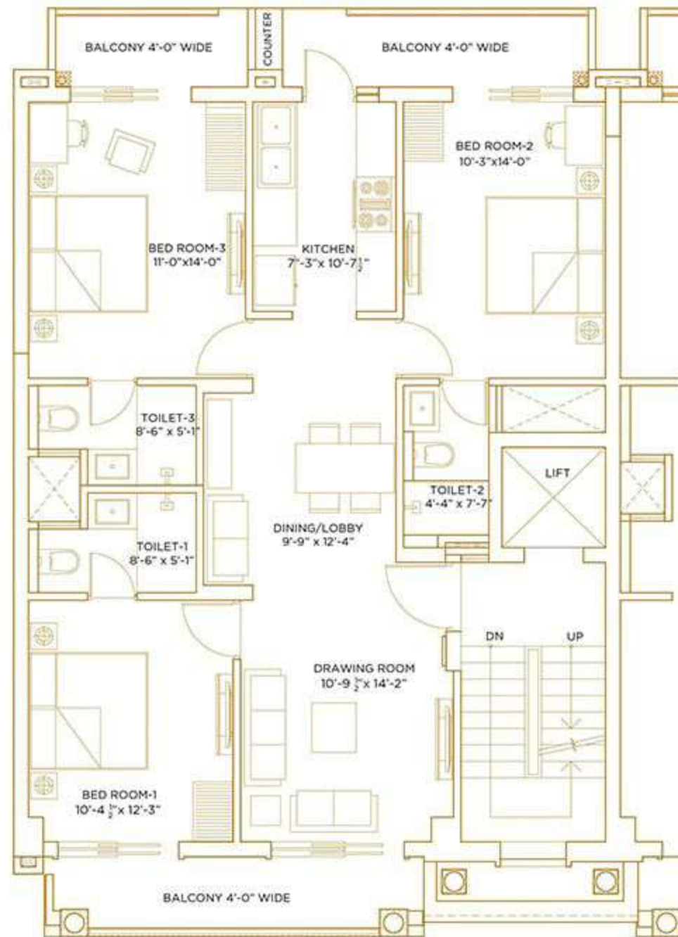
TYPICAL FLOOR PLAN SIZE = 30'-4.5" x 60'-0" 3BHK PREMIUM - 202.5 Square Yards
