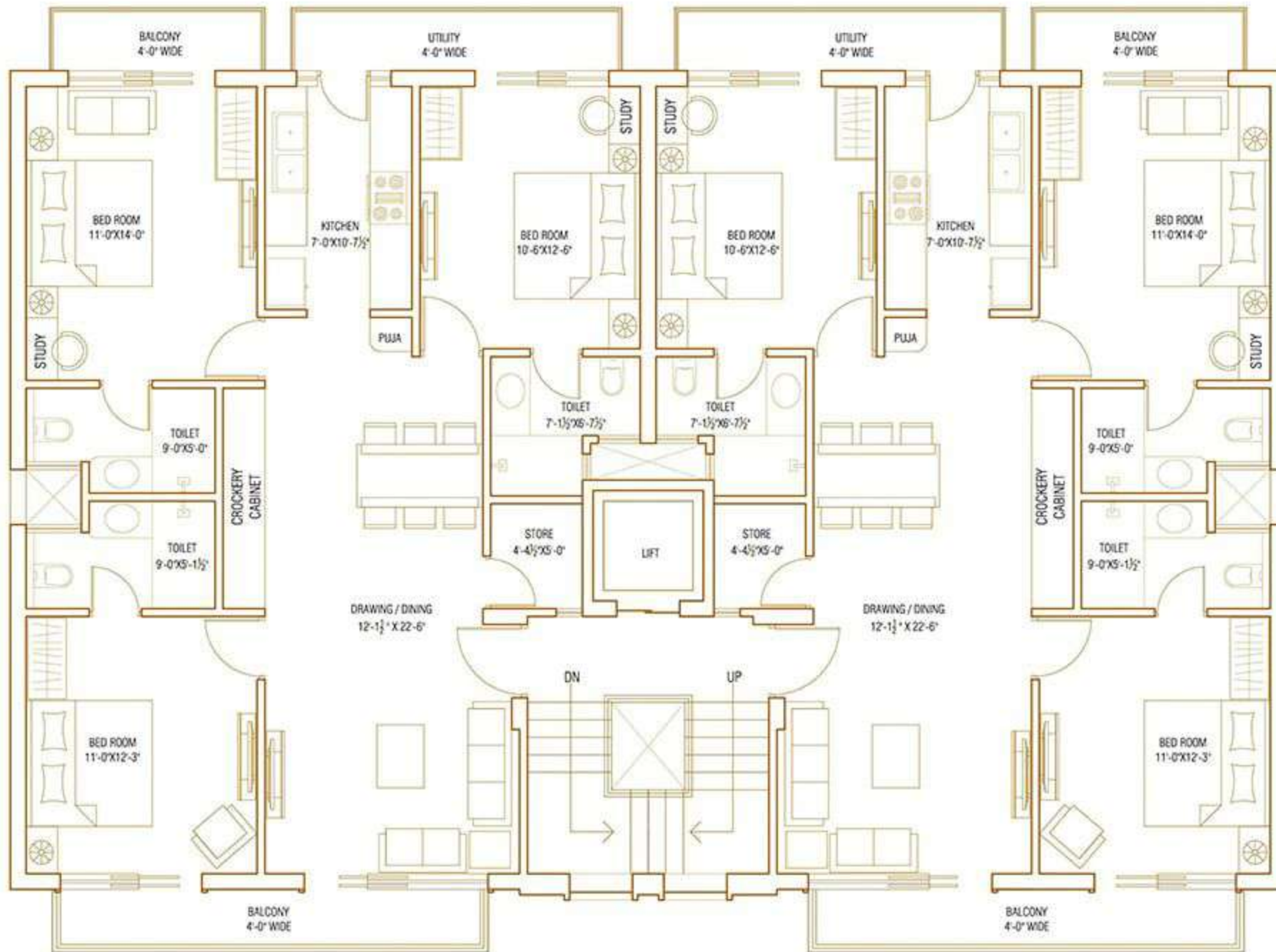
TYPICAL FLOOR PLAN SIZE = 30'-0" x 60'-0" 3BHK PREMIUM - 200 Yards
