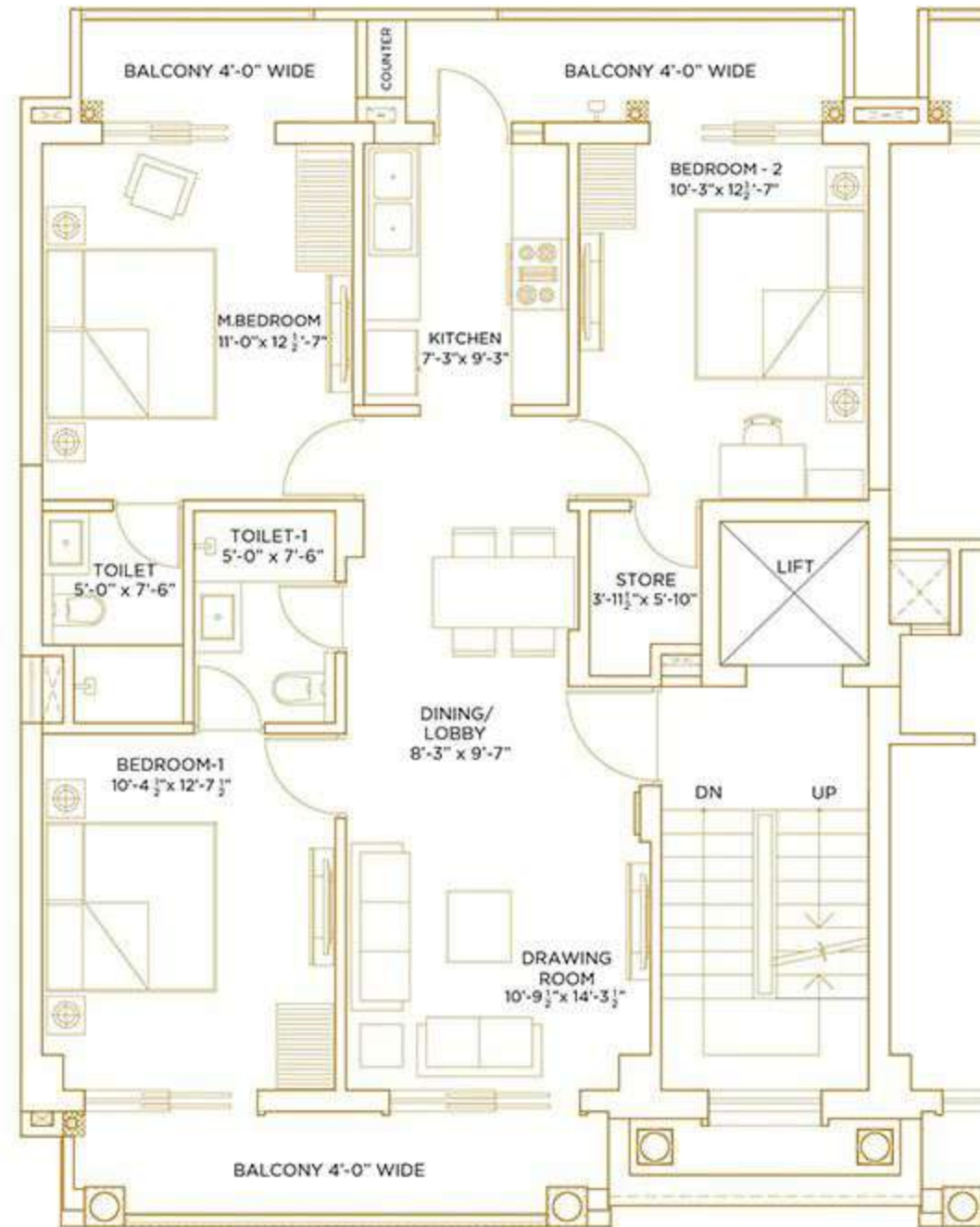
TYPICAL FLOOR PLAN SIZE = 30'-4.5" x 60'-0" 3BHK FLOOR - 202.5 Square Yards
